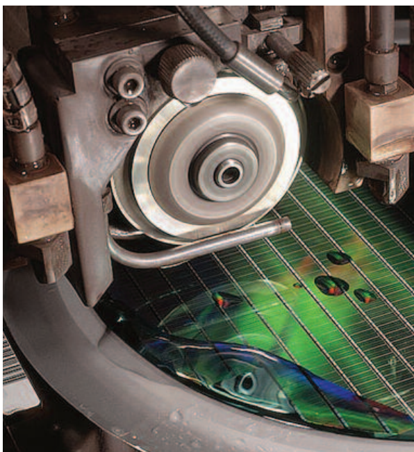
Die cutting process: One of the several hundred crucial steps in turning a wafer into a finished chip.
