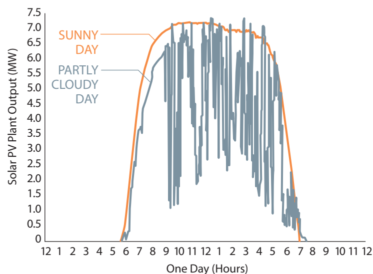
Variations in Solar PV Plant Output Actual Field Measurements – PV Solar Generation (MW)
